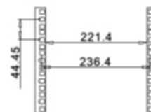
Mounting Dimension
